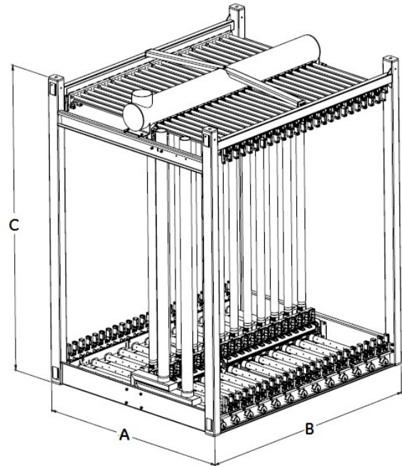
Figure 1: Example Drawing of Cassette
